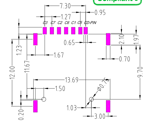
PCB LAYOYT
